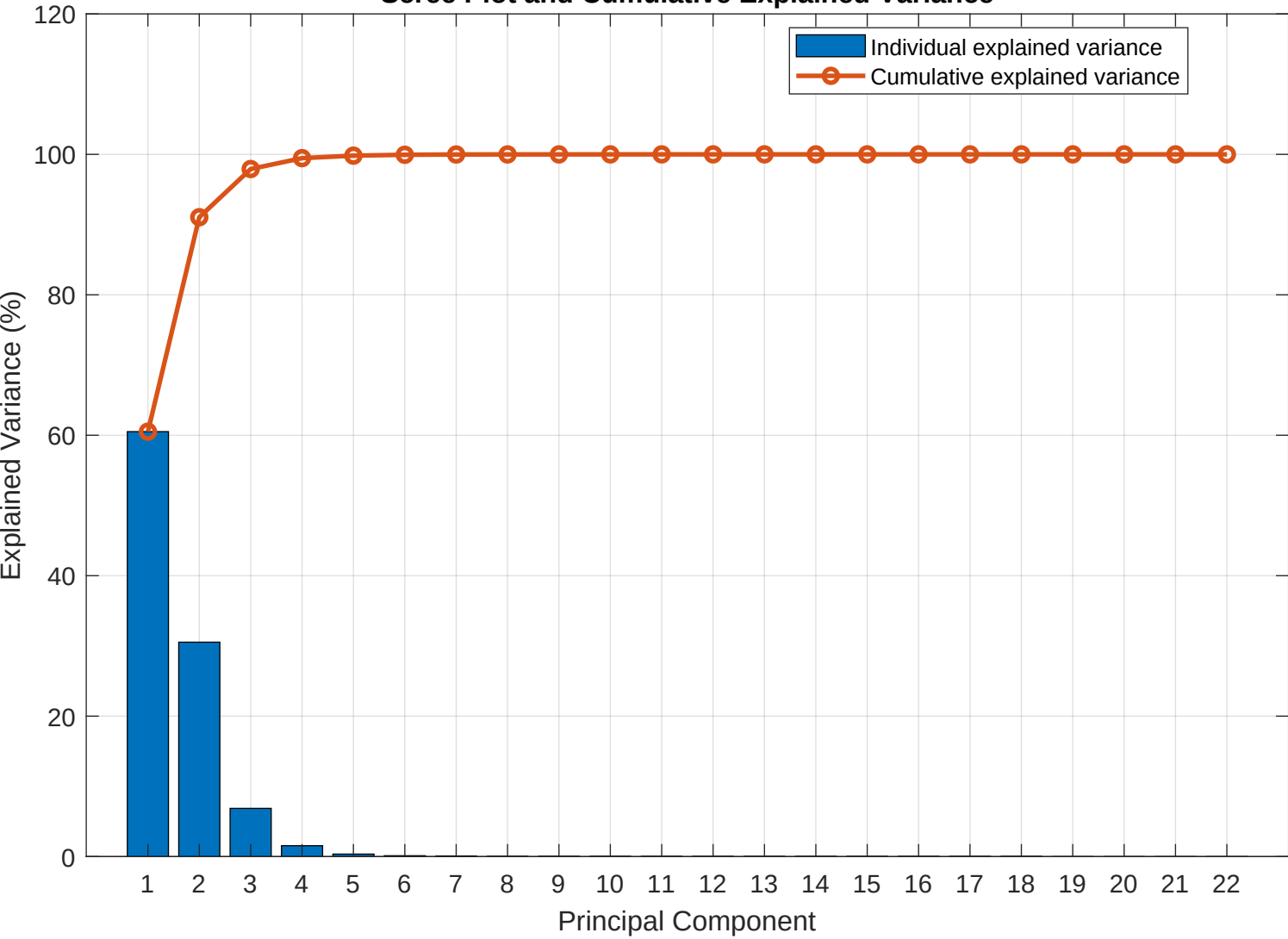
Scree Plot and Cumulative Explained Variance
